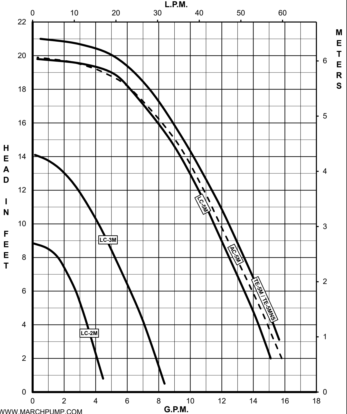
Family Curve (50Hz)
