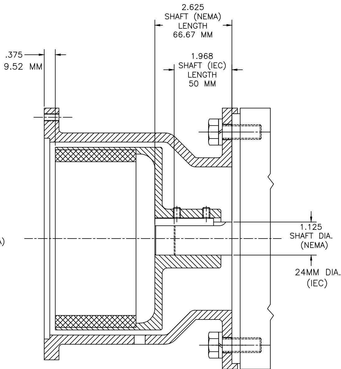
SERIES 8 PUMPS
