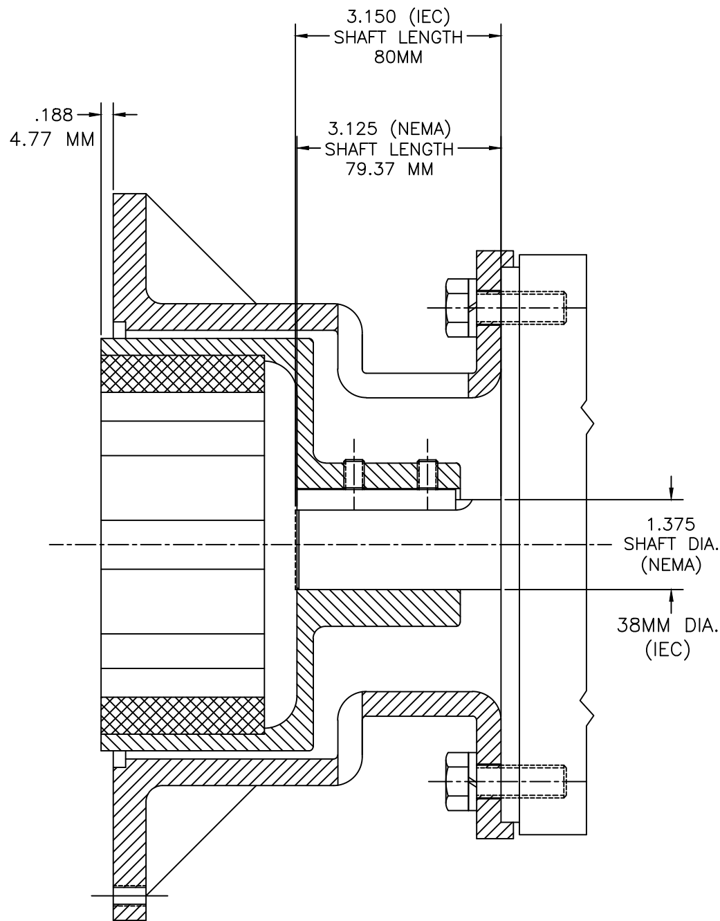
SERIES 10 PUMPS
