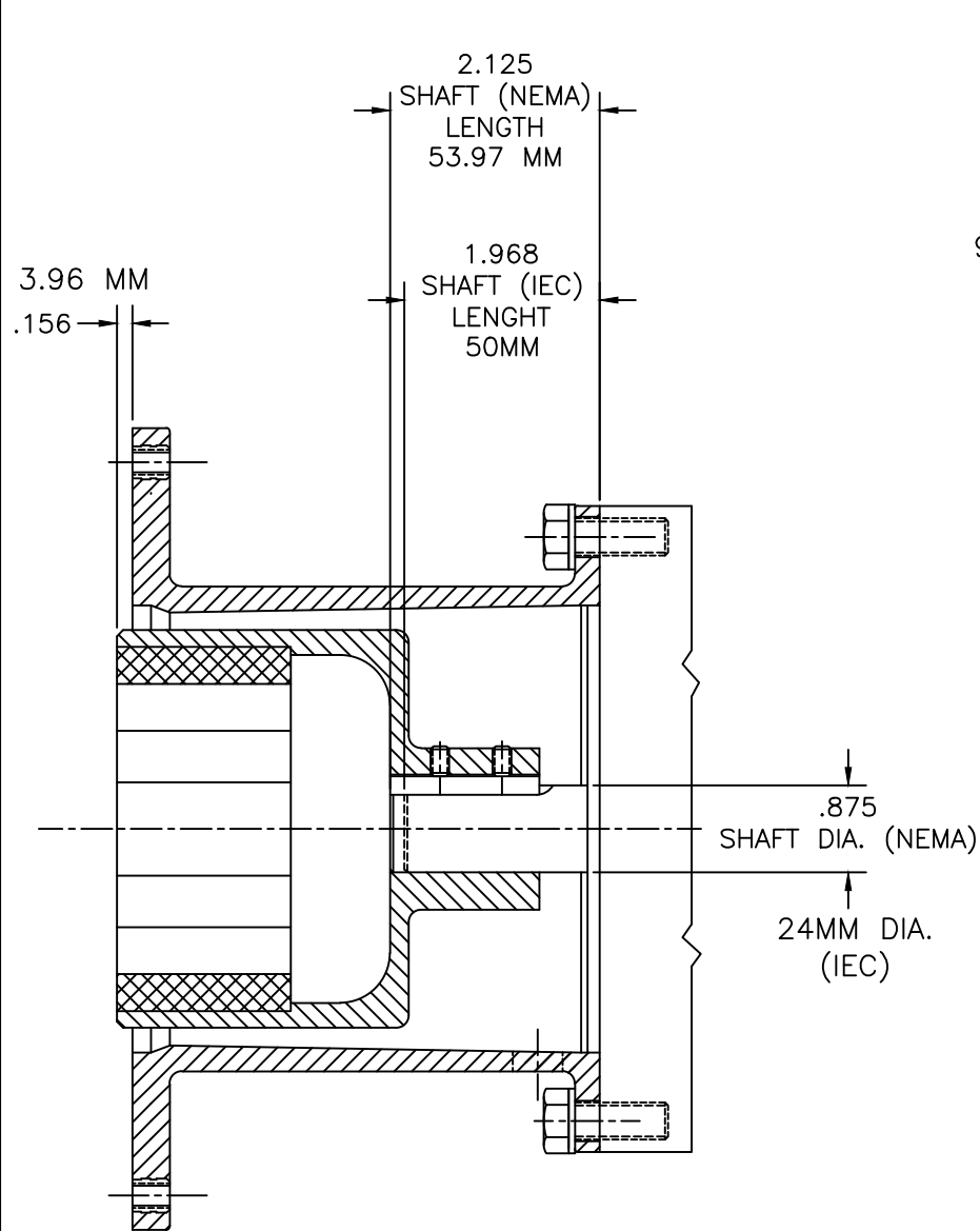
SERIES 7.5 PUMPS
